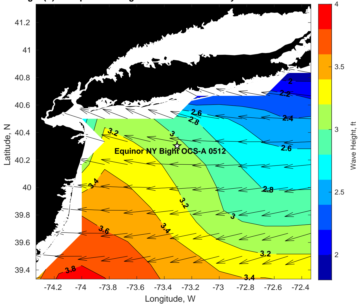
Wave Height (ft) for Equinor NY Bight OCS-A 0512 at 05-May-2024 12:00:00
